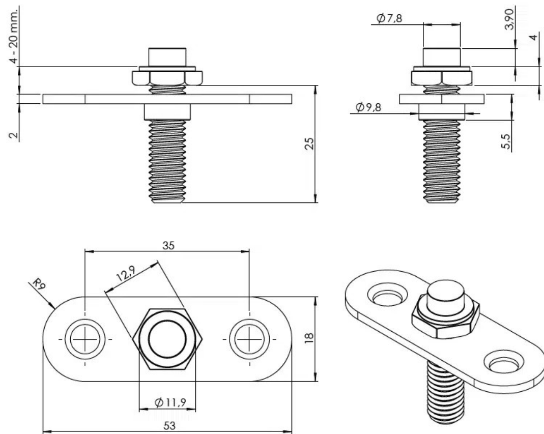
BOTTOM FITTING
