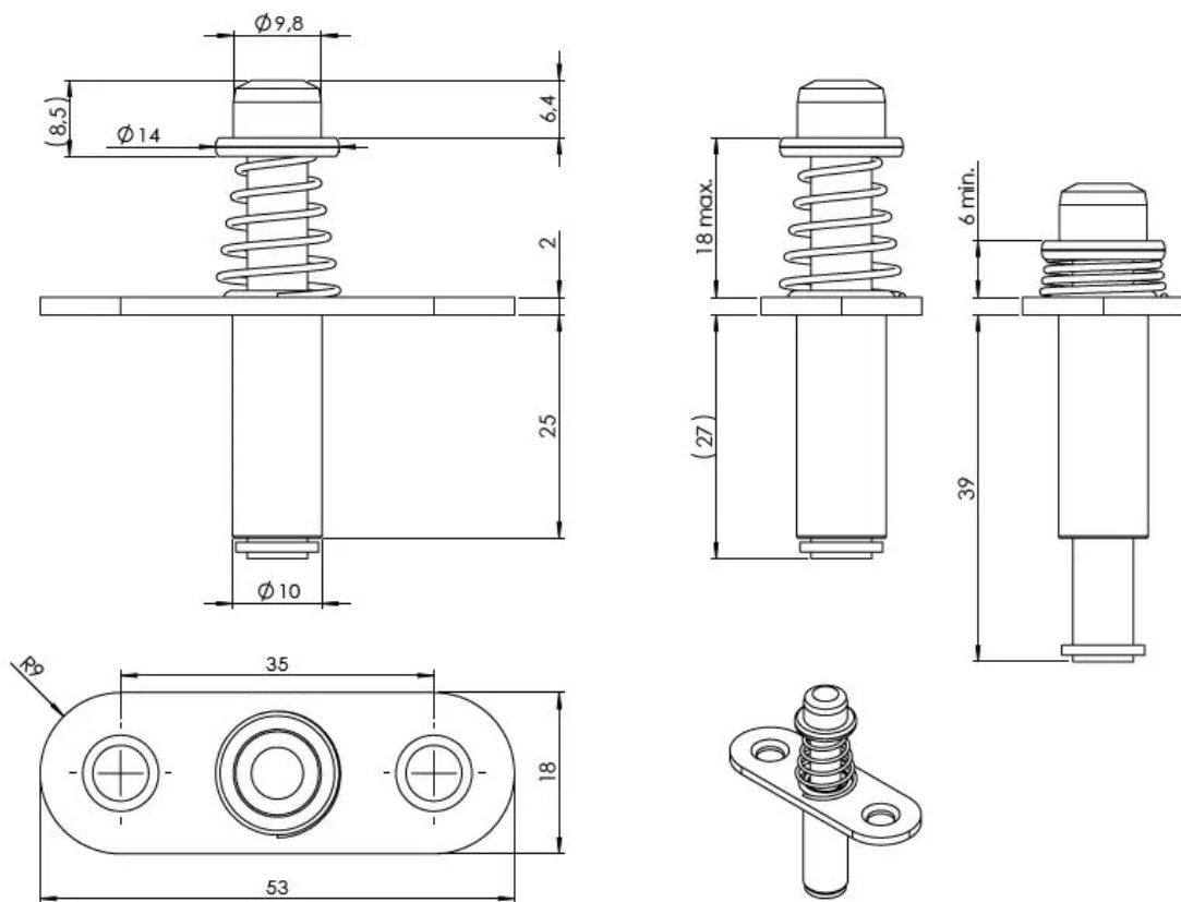
TOP FITTING
