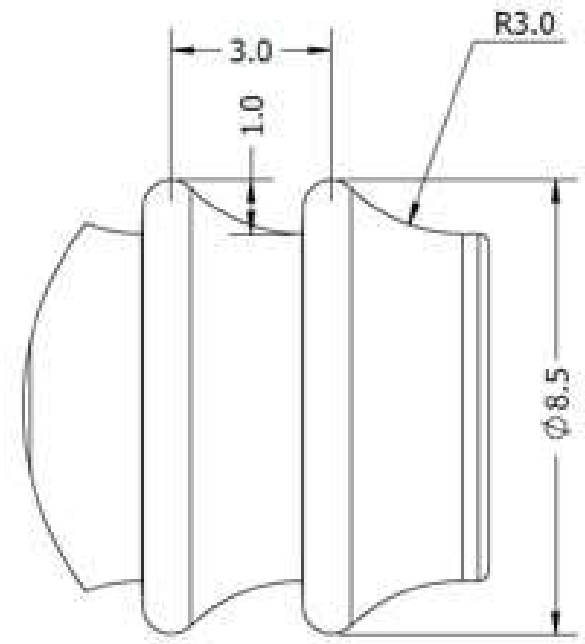
DETAIL A SCALE 8 : 1
