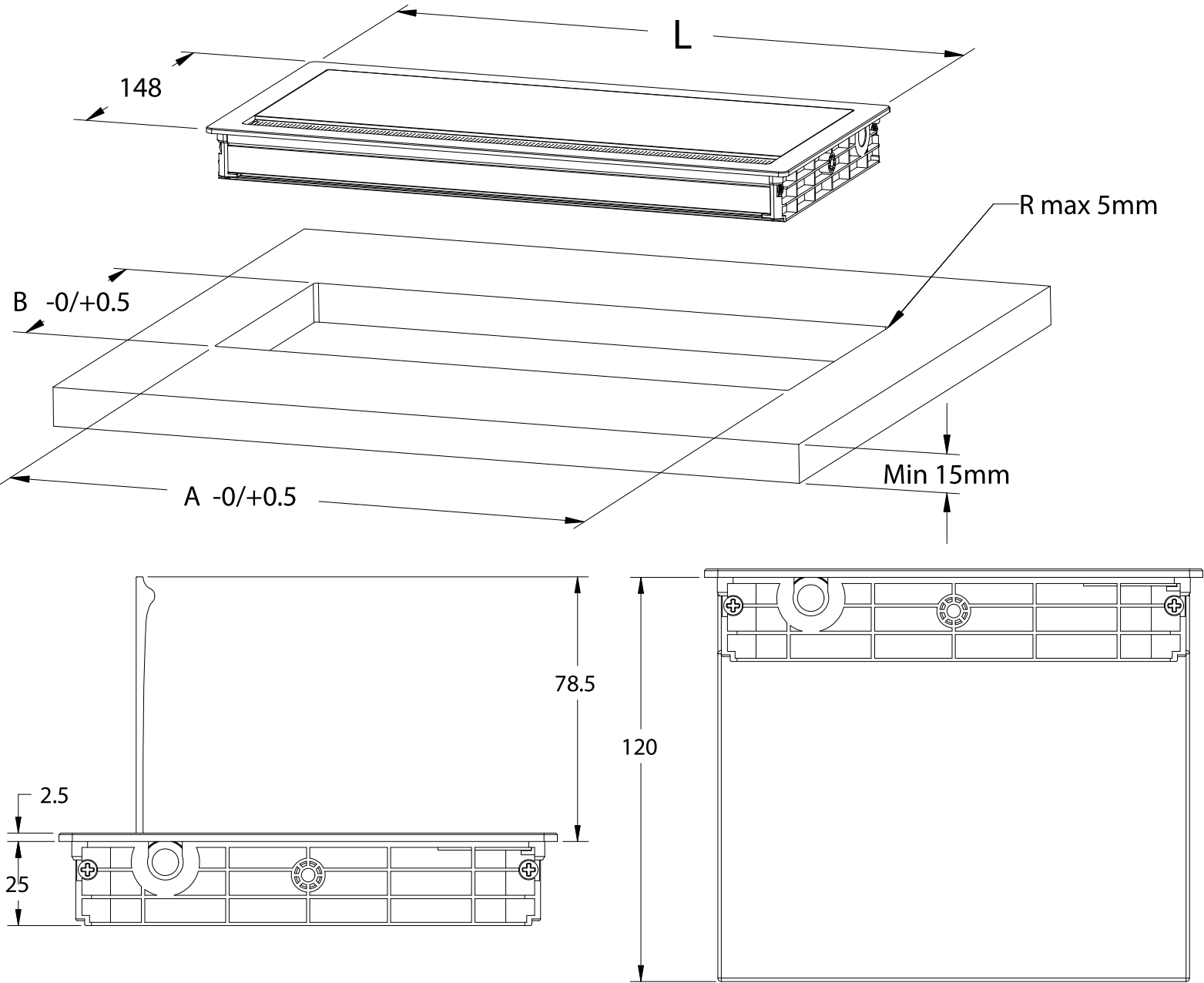
VASCA PORTA CAVI / CABLE TRAY
