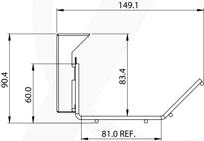
'PROFILE' DETAIL A SCALE 1 : 2
